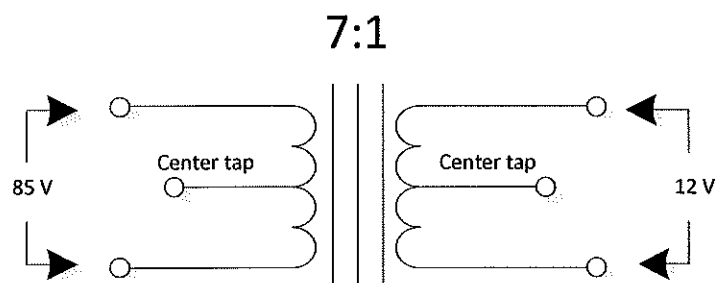
Schematic diagram of the 500 kV isolation transformer
