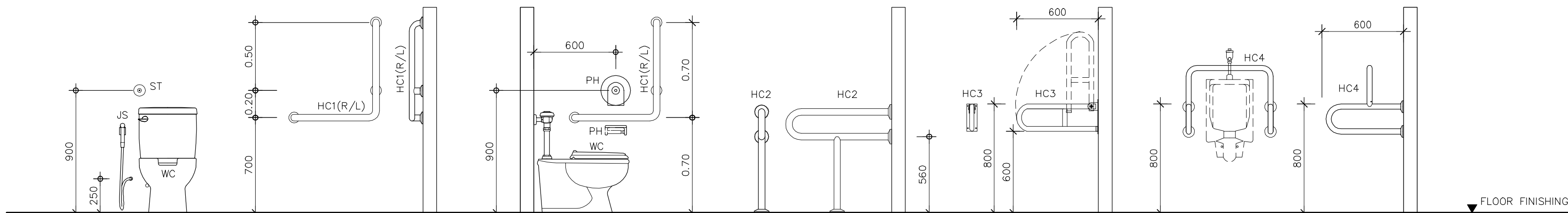
SANITARY WARE INSTALLATION STANDARDS
